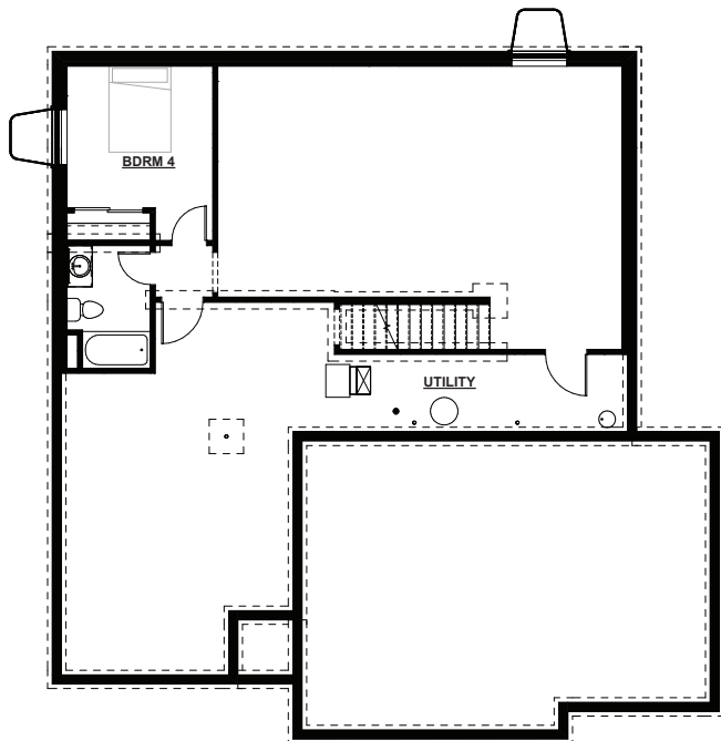
LOWER LEVEL
