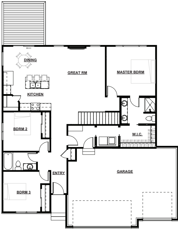
MAIN LEVEL
